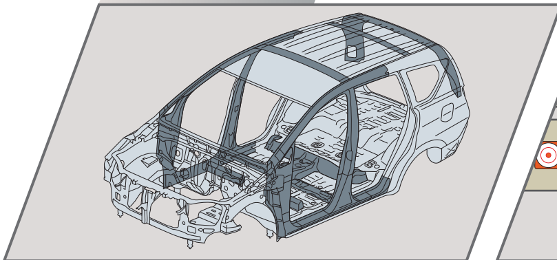
Impact Absorbing Body & Frame Structure The Innova's body structure is made of high-tensile steel sheets and supplementary materials to absorb impact in the event of a collision.
